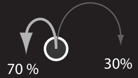
Example intensity division between bins for one datapoint
