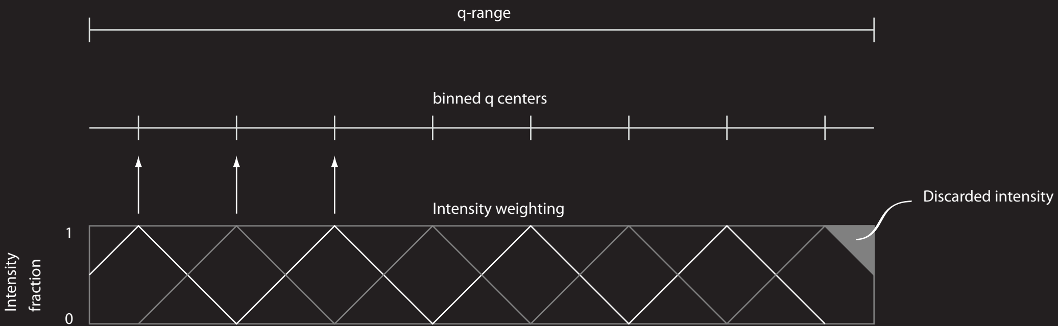
Example intensity division between bins for one datapoint
